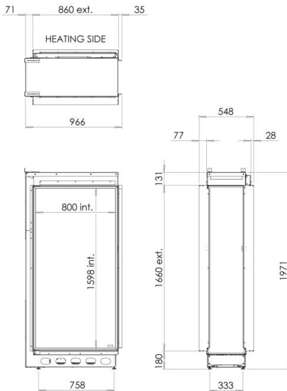
Dimensional Drawing e-Matrix 800/1600 ST
